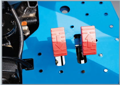
Dual pedal, 3 range HST (HST model) Easier and more comfortable than rocker pedals. Includes cruise control.
